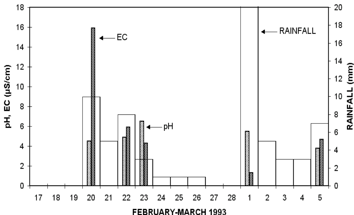
Fig. 4. Rainfall, electrical conductivity (EC) and pH of rainwater, in the period February-March 1993.
