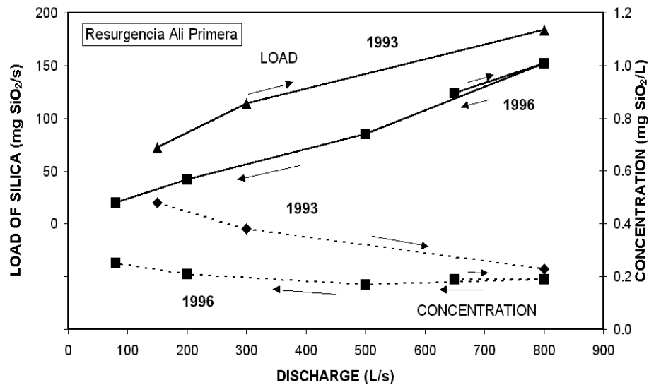
Fig. 12. Relationship between dissolved silica load and SiO 2 concentration to discharge, at Resurgencia Alí Primera.
