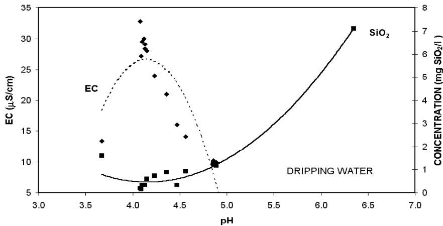
Fig. 8. Relationship between electrical conductivity (EC) (rhombuses) and dissolved SiO 2 concentrations (squares) vs. pH, in cave dripping water.
