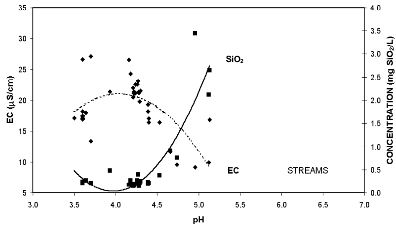
Fig. 7. Variations of electrical conductivity (EC) and pH in the stream of Sima Auyàn-tepi Norte 2.
