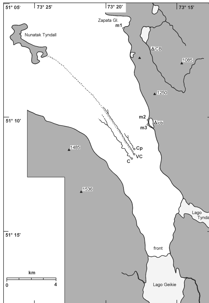
Fig. 1- Sketch map of Glacier Tyndall, with the position of major streams and moulins: C) moulin “Capo”; VC) moulin “Vice-capo”; Cp) moulin “Capino”; CB) base camp; cb) advanced base camp; m1-m2-m3) marginal contact caves.
