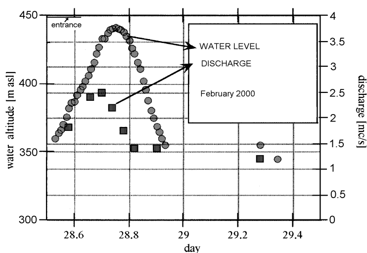
Fig. 3 – Immobilized and removed water discharge vs time in Vicecapo.
